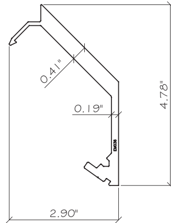
E43 CORNER MULLION ALUM. 6063-T6
