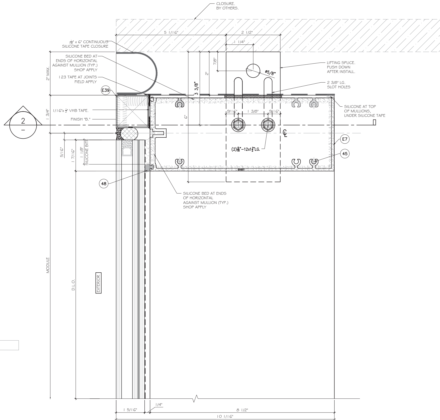
1 D1 SECTION DETAIL SCALE 1'-0"=1'-0"
