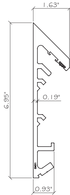
E4 FEMALE MULLION GW-7000-168 ALUM. 6063-T6
