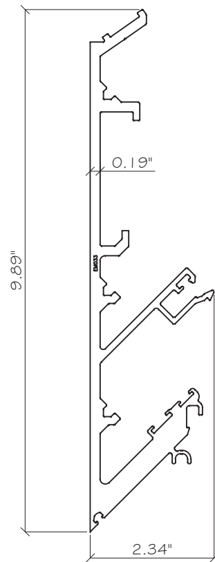
E42 CORNER MULLION ALUM. 6063-T6
