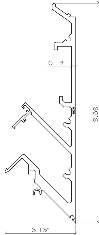
E44 CORNER MULLION ALUM. 6063-T6
