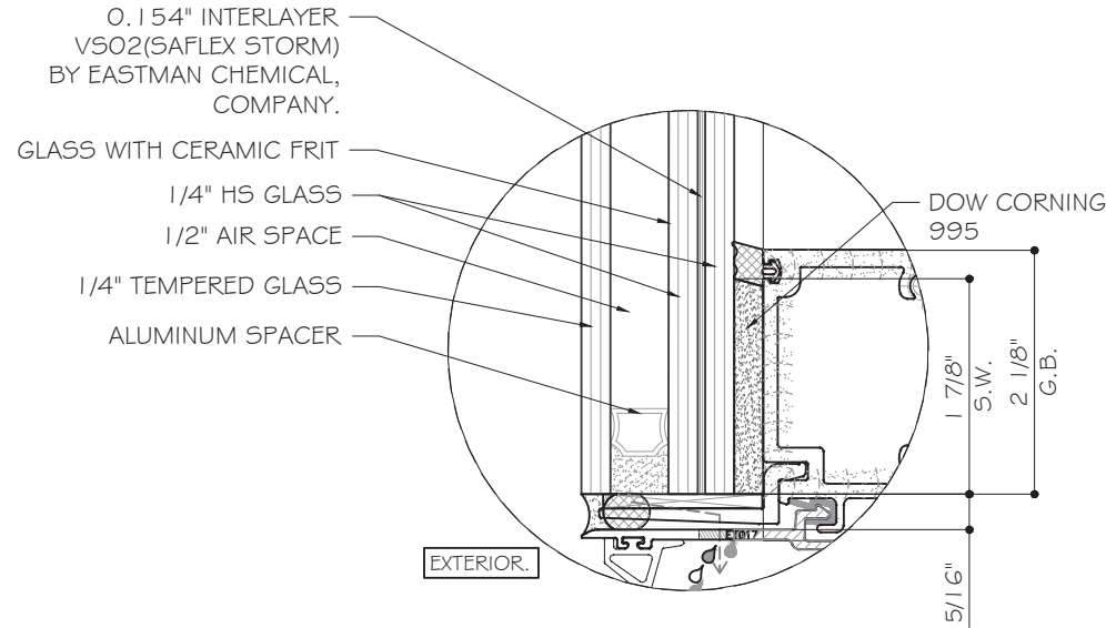
GS2 GLASS TYPE 'GS2' 3/8" NOMINAL OVERALL LARGE MISSILE IMPACT LEVEL E SPANDREL GLASS
