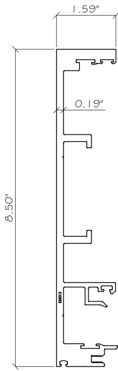
E1 FEMALE MULLION GW-7000-190 ALUM. 6063-T6
