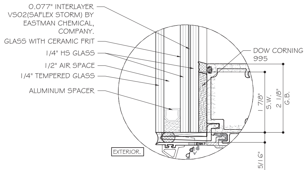
GS1 GLASS TYPE 'GS1' 5/16" NOMINAL OVERALL LARGE MISSILE IMPACT LEVEL D SPANDREL GLASS
