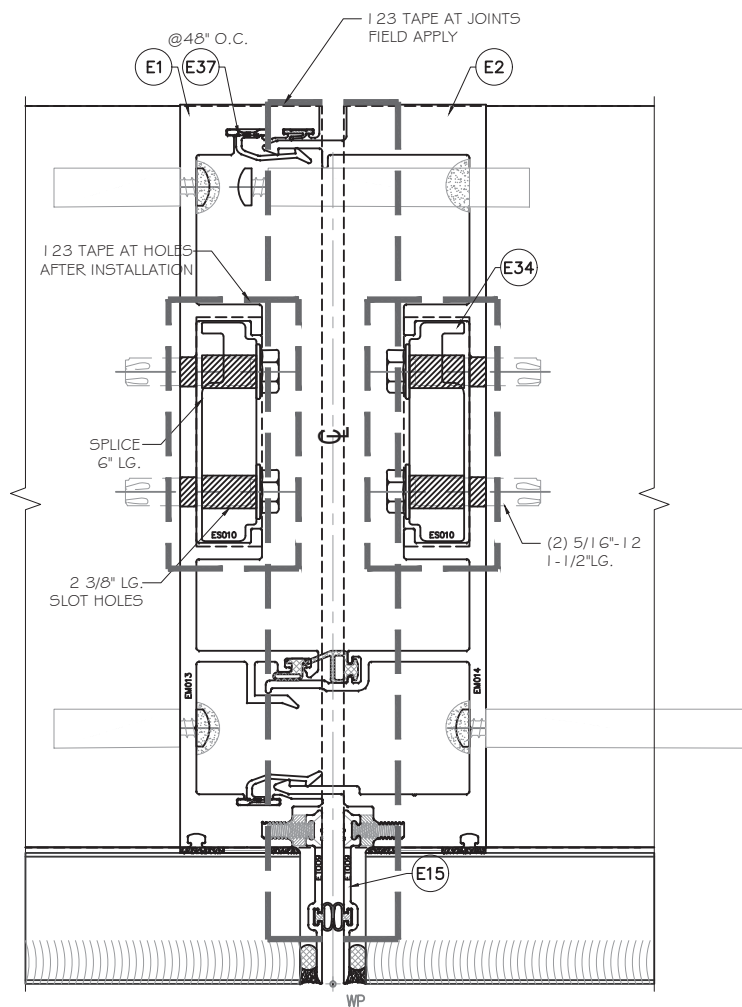
2 - DETAIL SCALE 1'-0"=1'-0"
