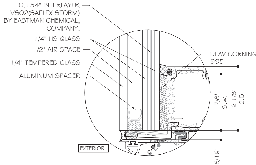
G2 GLASS TYPE 'G2' 3/8" NOMINAL OVERALL LARGE MISSILE IMPACT LEVEL E
