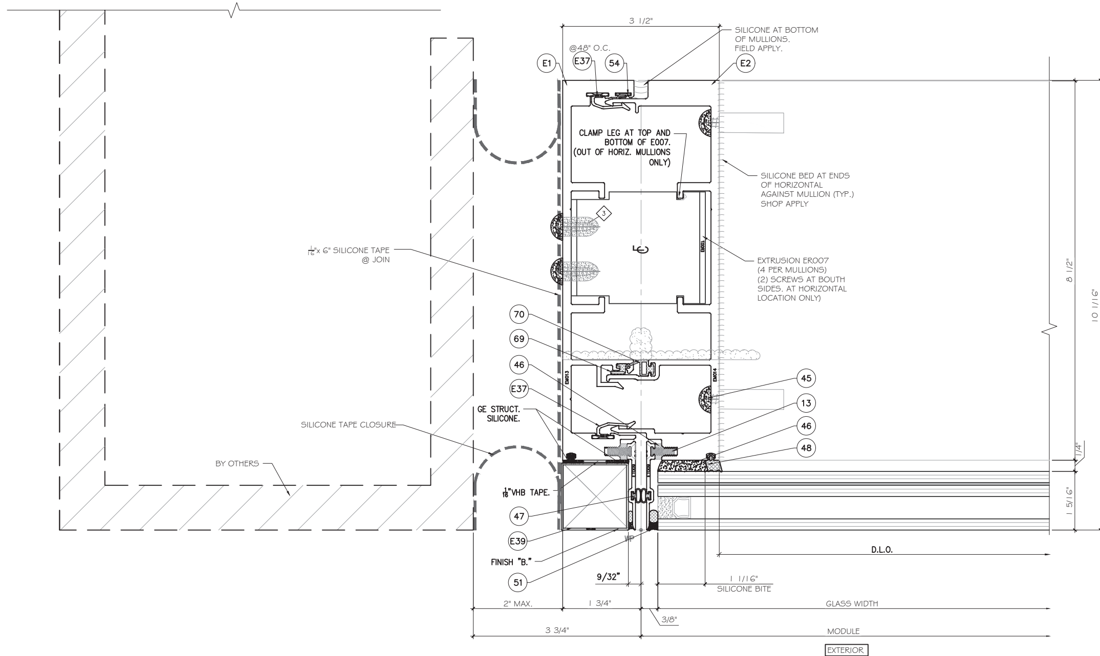
1 PLAN DETAIL D12 SCALE 1'-0"=1'-0"
