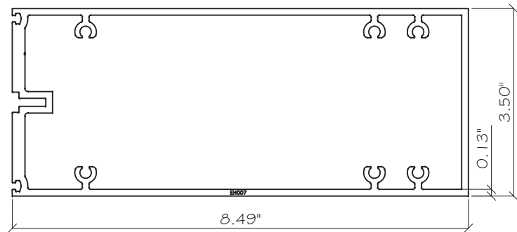
E7 INTERMEDIATE HORIZONTAL ALP-039 ALUM. 6063-T6
