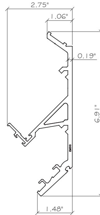
E5 MALE MULLION GW-7000-169 ALUM. 6063-T6
