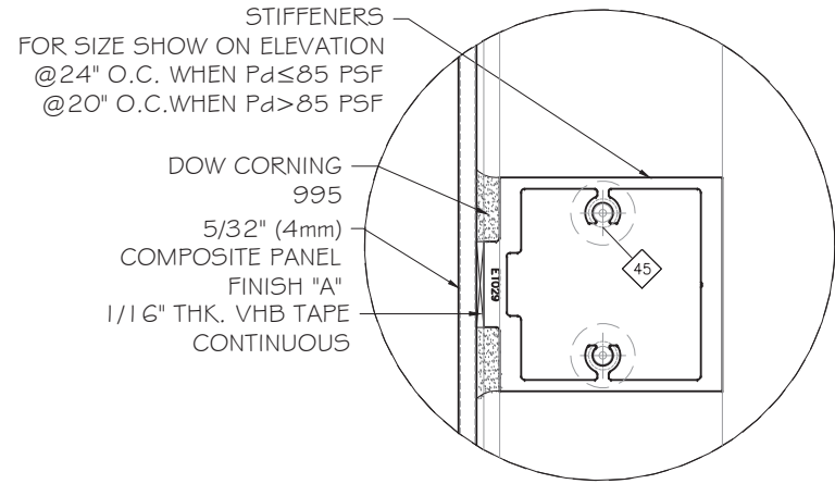
PI 5/32" (4mm) COMPOSITE PANEL LARGE MISSILE IMPACT LEVEL E
