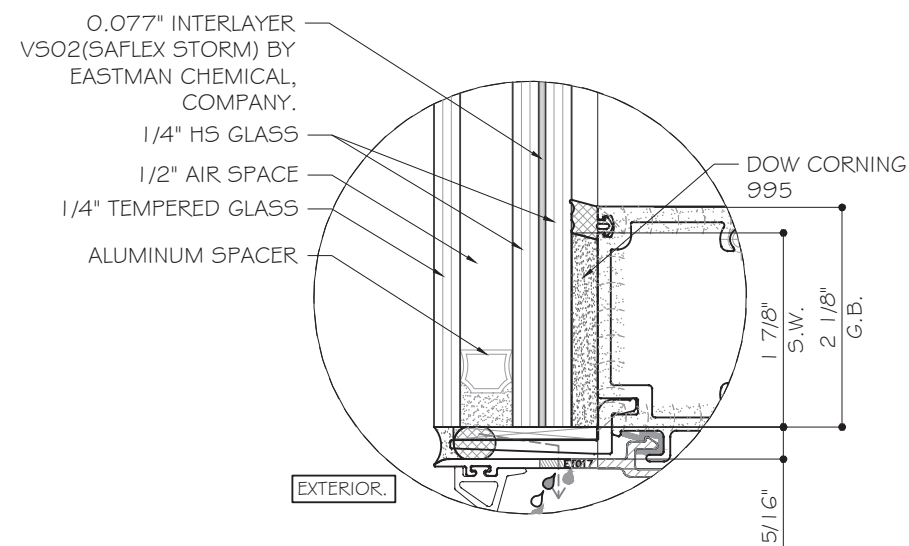
G1 GLASS TYPE 'G1' 5/16" NOMINAL OVERALL LARGE MISSILE IMPACT LEVEL D
